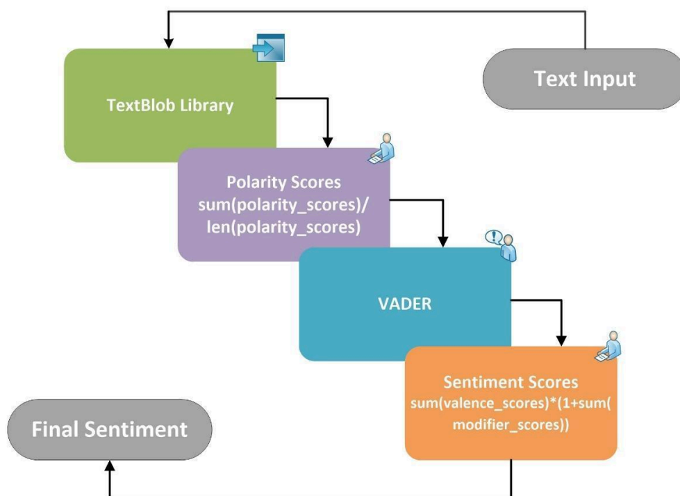
Figure 2. Process of sentiment analysis
