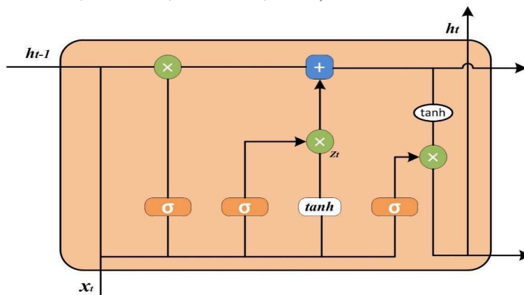
Figure 3. LSTM schematic diagram
