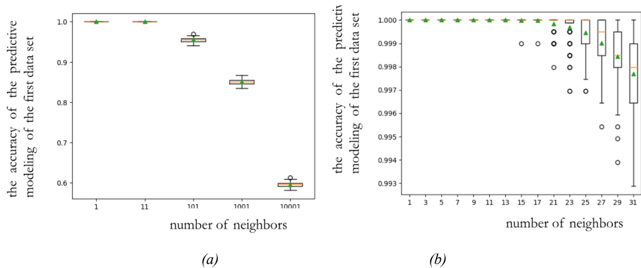
(a) (b) Figure 6. Accuracy vs. neighbors (dataset1)
