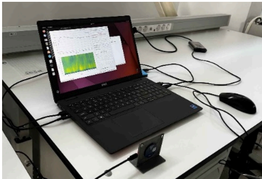
Figure 2. The minimum hardware configuration required to test
