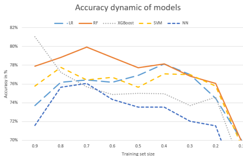
Figure 2. Impact of the training set size on model accuracy.
