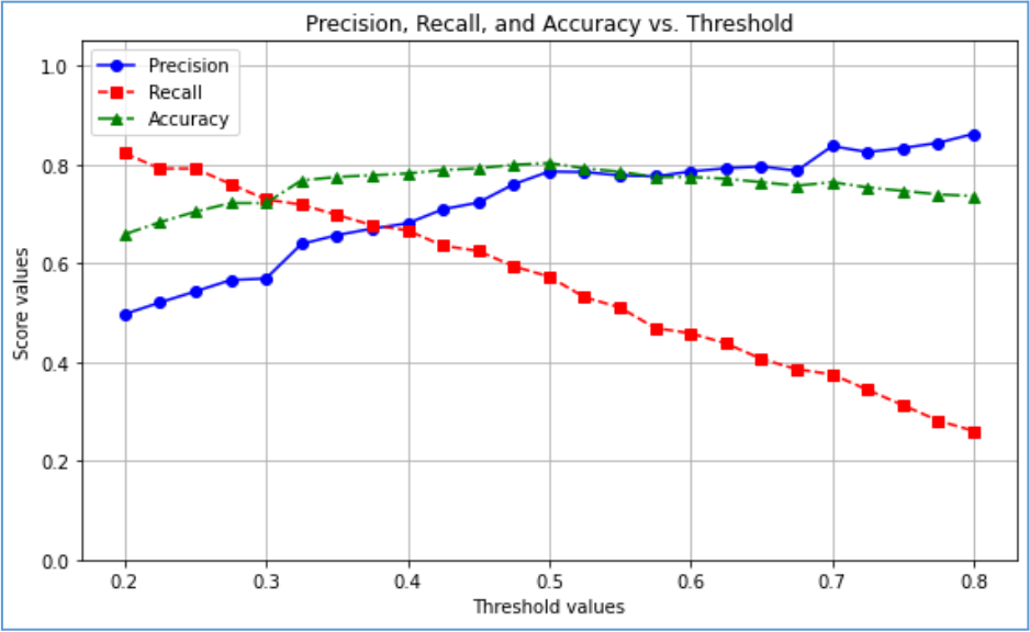
Figure 3. Random Forest model performance across different threshold values
