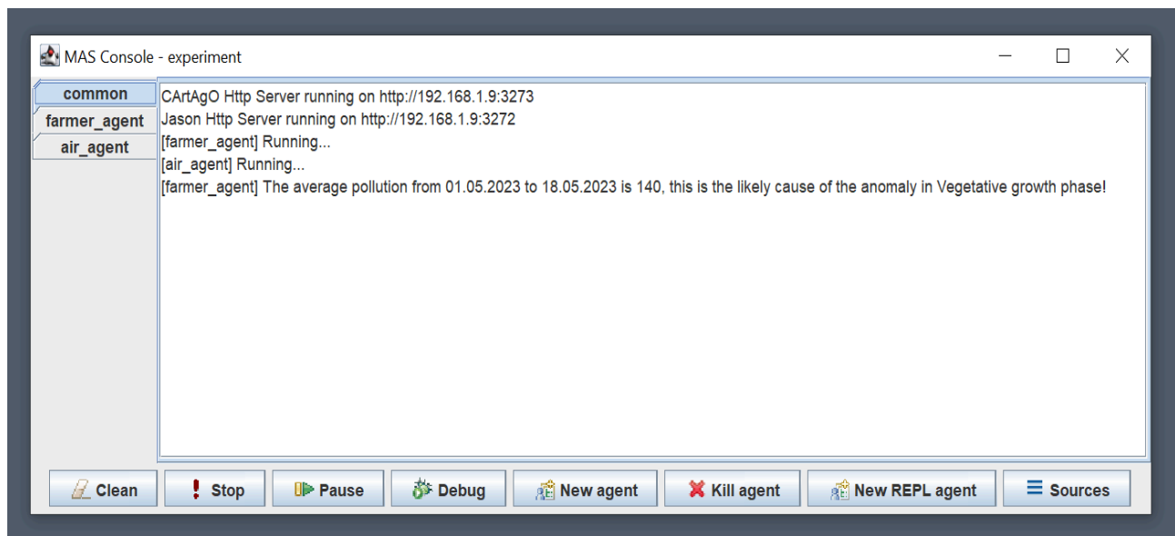
Figure 8. Example interaction session between the two agents
