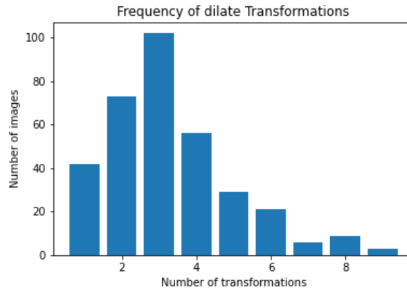
Figure 12. Histogram for the number of dilate operations
