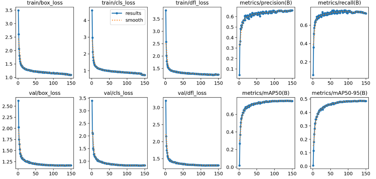
Figure 5. Training and Validation Graph.
